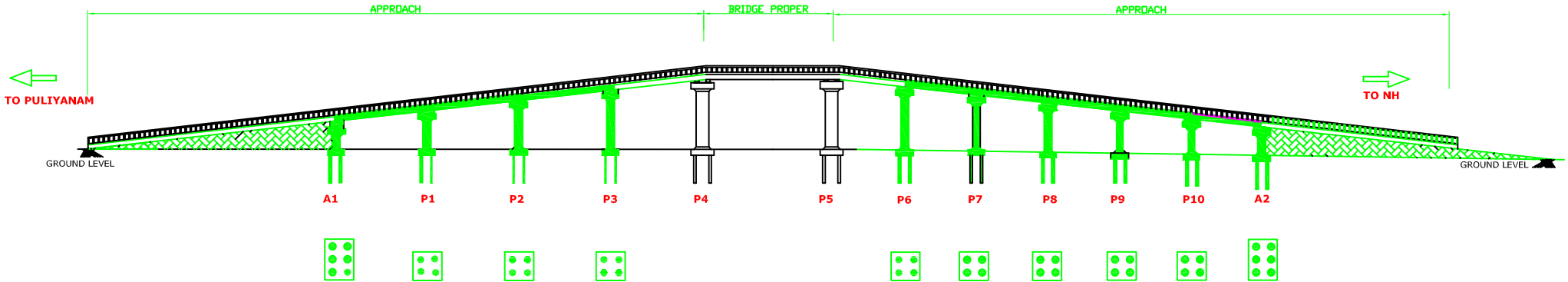
PILE FOUNDATION
